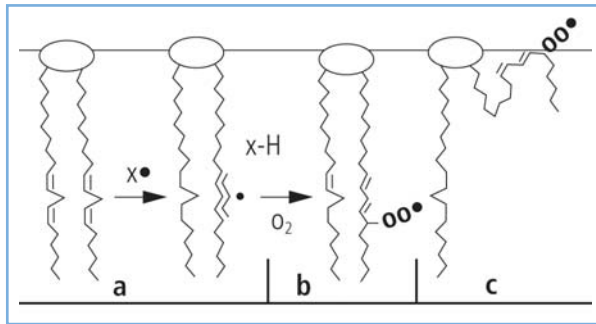
Abb. 9: Lipidperoxidation.
